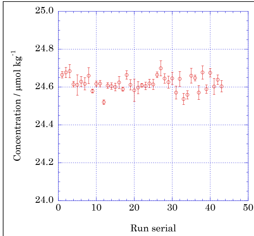
Figure 4.2-12 Time series of CRM-BW of nitrate in MR15-03.
