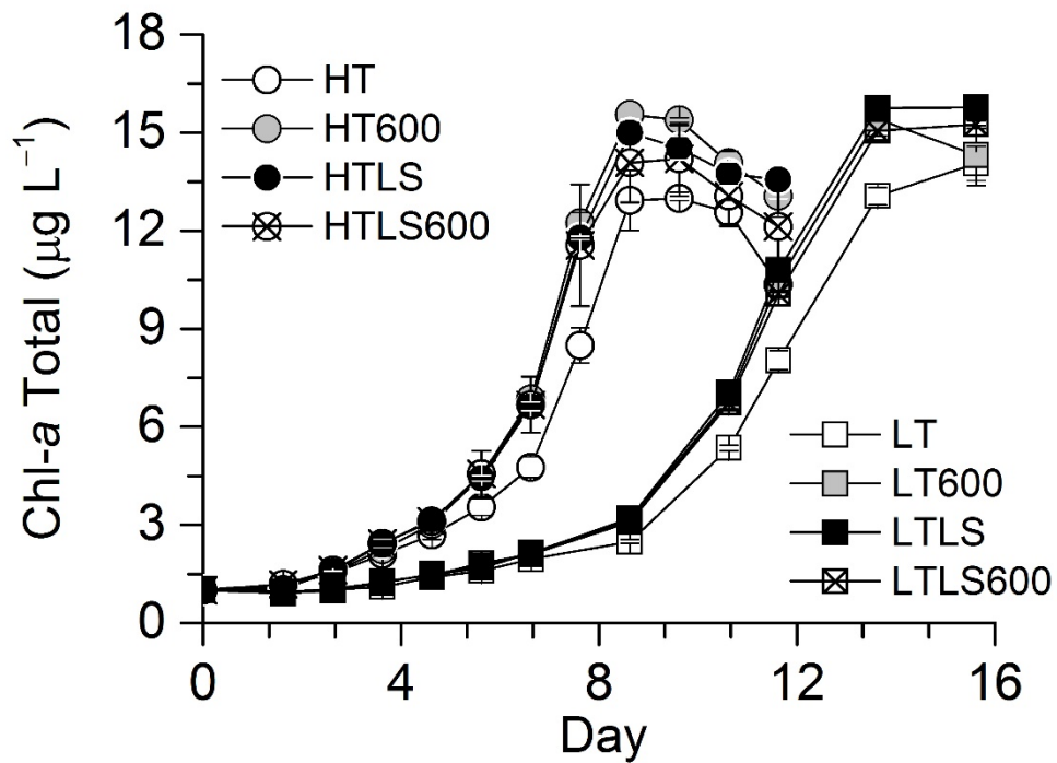
Fig. 4.19.2. Temporal change in chlorophyll- a concentration during the incubation.
