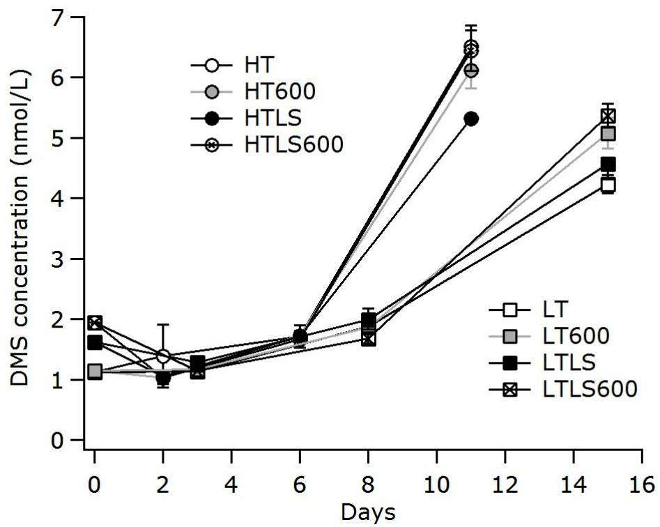
Fig. 4.19.3. Temporal change in DMS concentration during the incubation.
