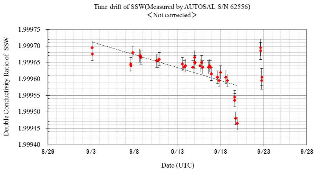
Fig. 3.7-1 History of double conductivity ratio for the Standard Seawater batch P157 in the salinometer S/N 62556 (before correction)
