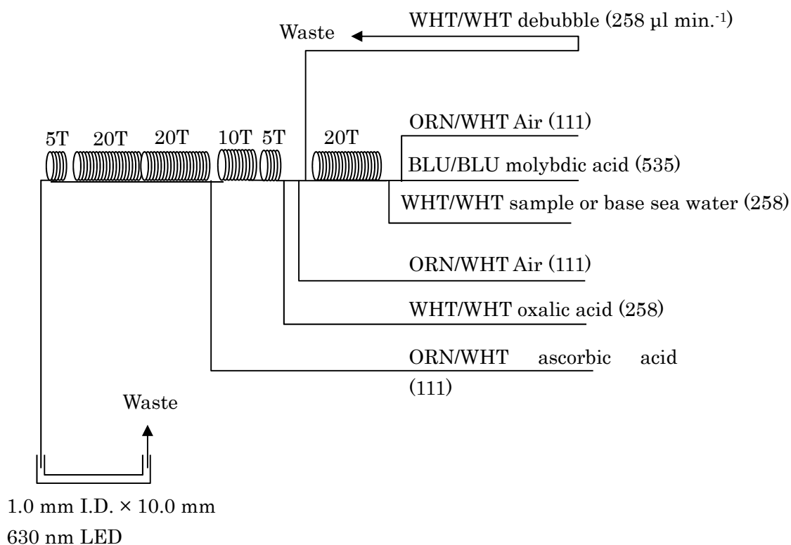
Figure 4.2-3 SiO 2 (3ch.) Flow diagram.
