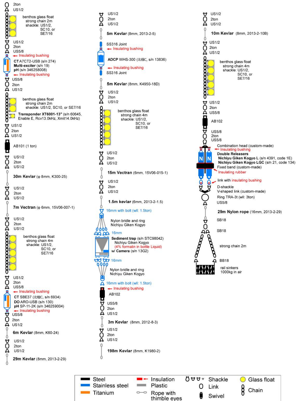
Fig. 4.21-5: The design of sediment trap mooring NHC15t.
