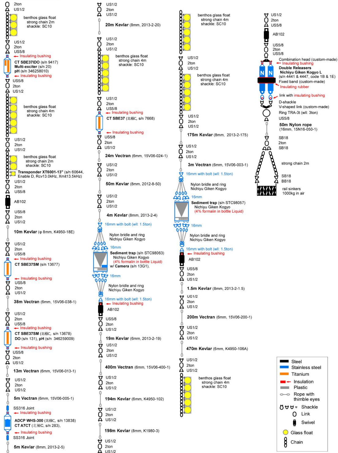
Fig. 4.21-3: The design of sediment trap mooring NBC15t.
