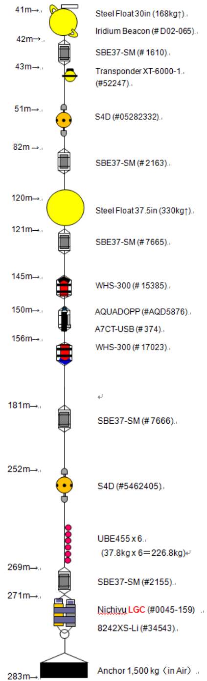
Figure 3.9-1: Diagrams of deployed moorings (BCW-15, BCE-15, and BCC-15).
