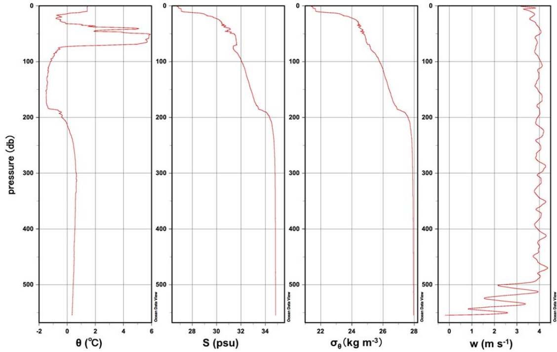
Figure 3.3-2: Typical profiles from U-CTD observation of (a) potential temperature \theta (deg-C), (b) salinity S (practical salinity unit), (c) potential density \sigma_\theta ( \text{kg m}^{-3} ), and (d) descending rate w ( \text{m s}^{-1} ) at a station of u003c01, positioned off the Barrow Canyon.
