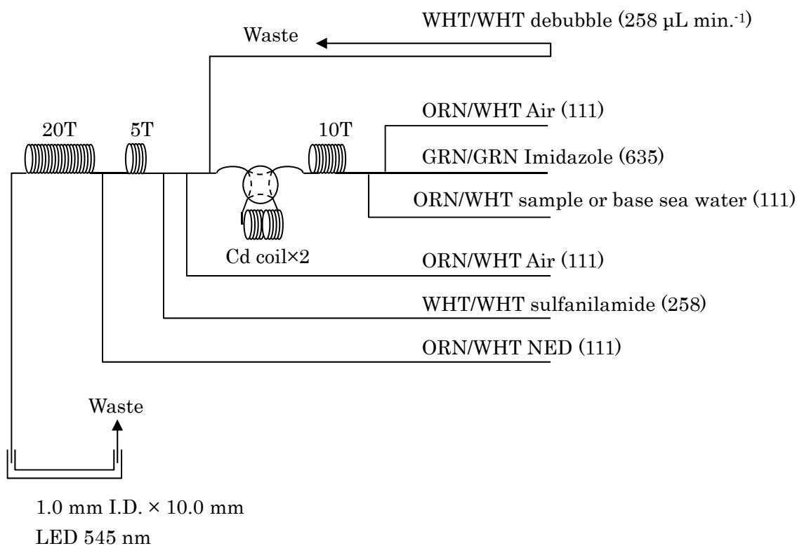
Figure 4.2-1 \text{NO}_3+\text{NO}_2 (1ch.) Flow diagram.
